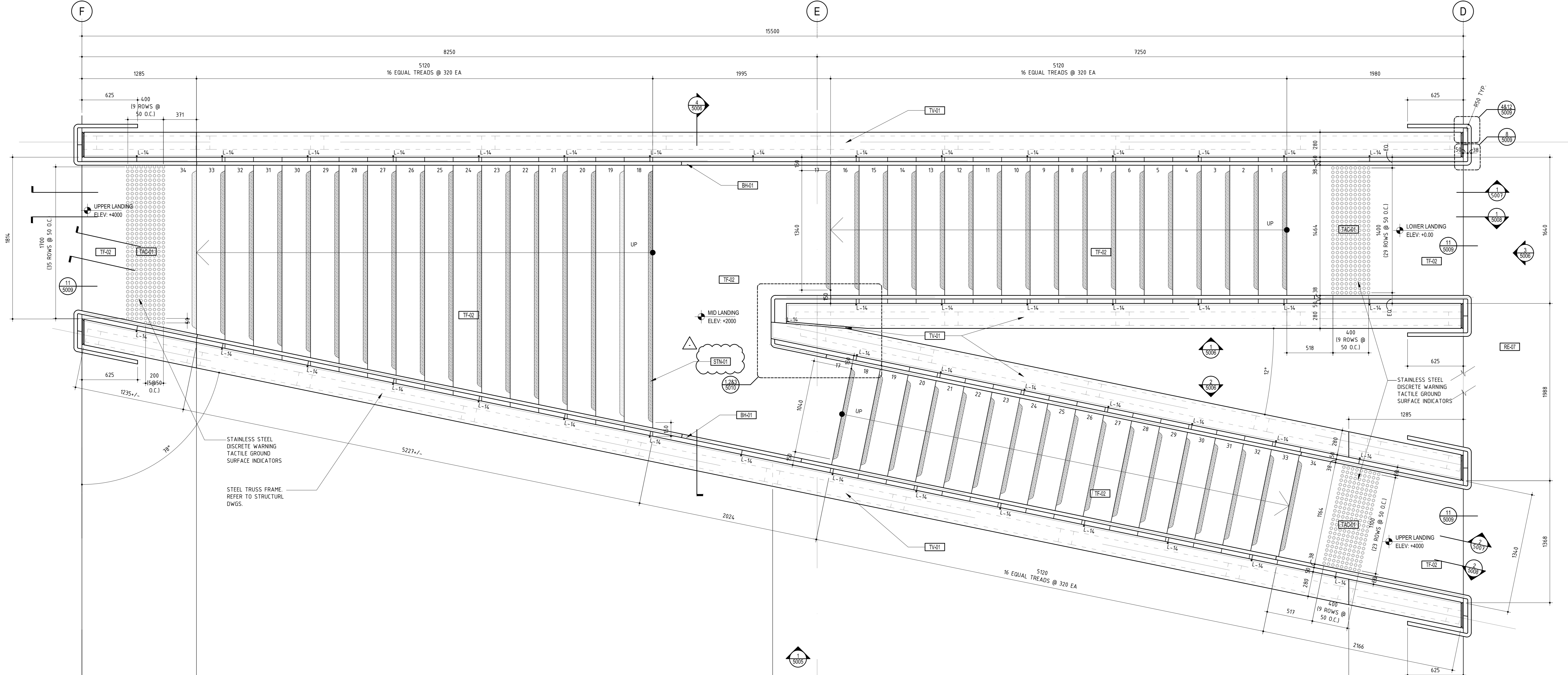
01 ENLARGED PLAN OF TYPICAL 000H STAIR SCALE 1:20
